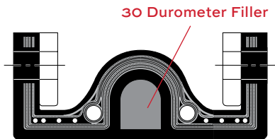
OPTIONAL FILLED ARCH CONSTRUCTION
